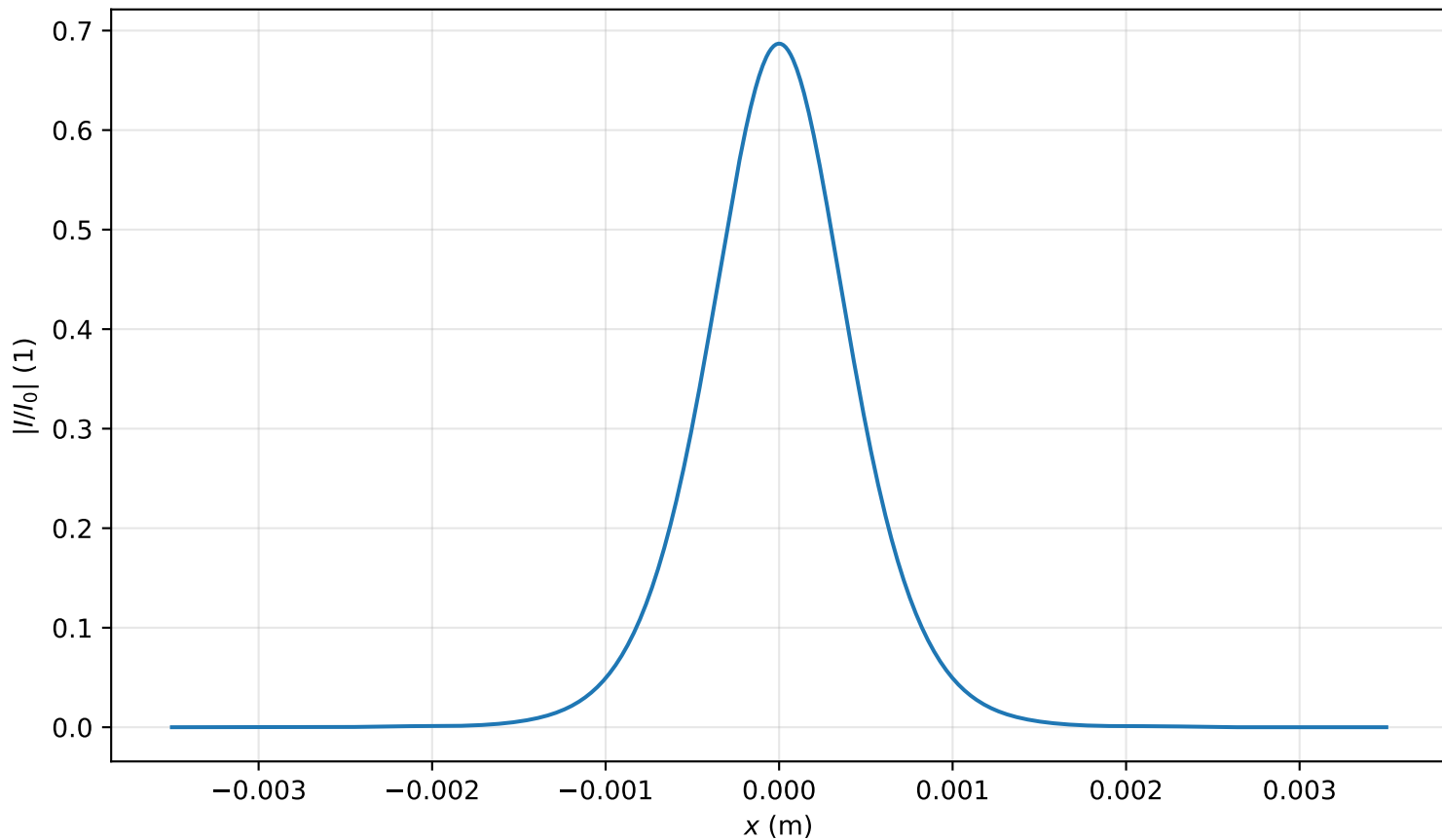
Intensity profile I(x, y = 0, z = 3.662m)/I_0 , P_{in}=0.7P_{cr} , artificial time
